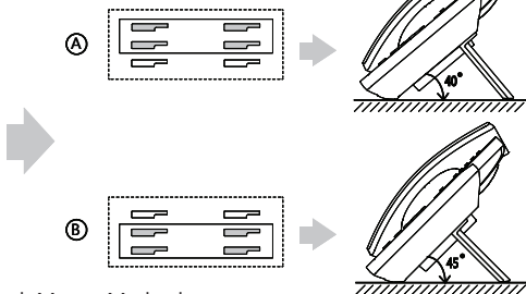
Desk Mount Method
